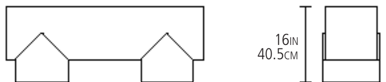
ELEVATIONS
