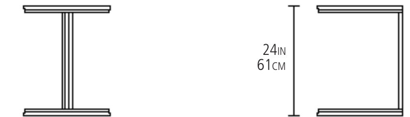
ELEVATIONS
